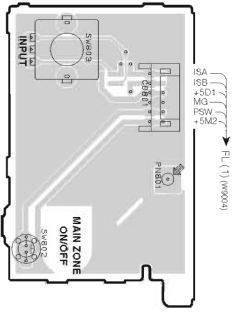
OPERATION (1) P.C.B. (Side A)
