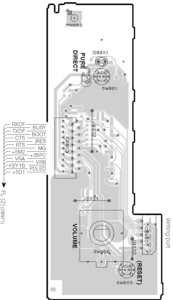
OPERATION (2) P.C.B. (Side A)
